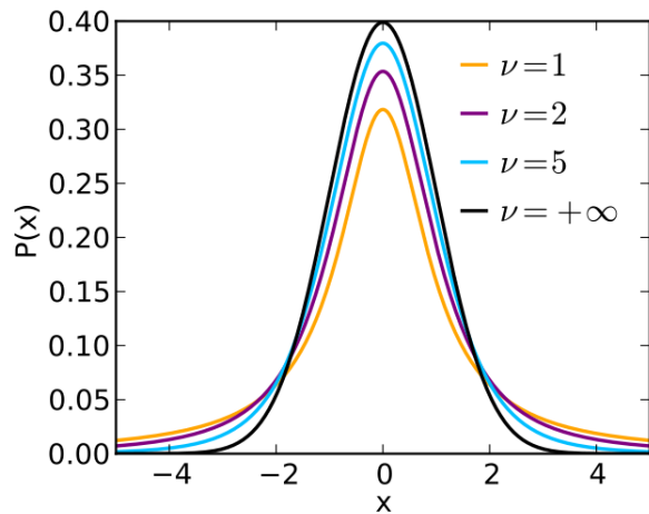
t distribution
