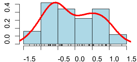
Fat tailed distributio
